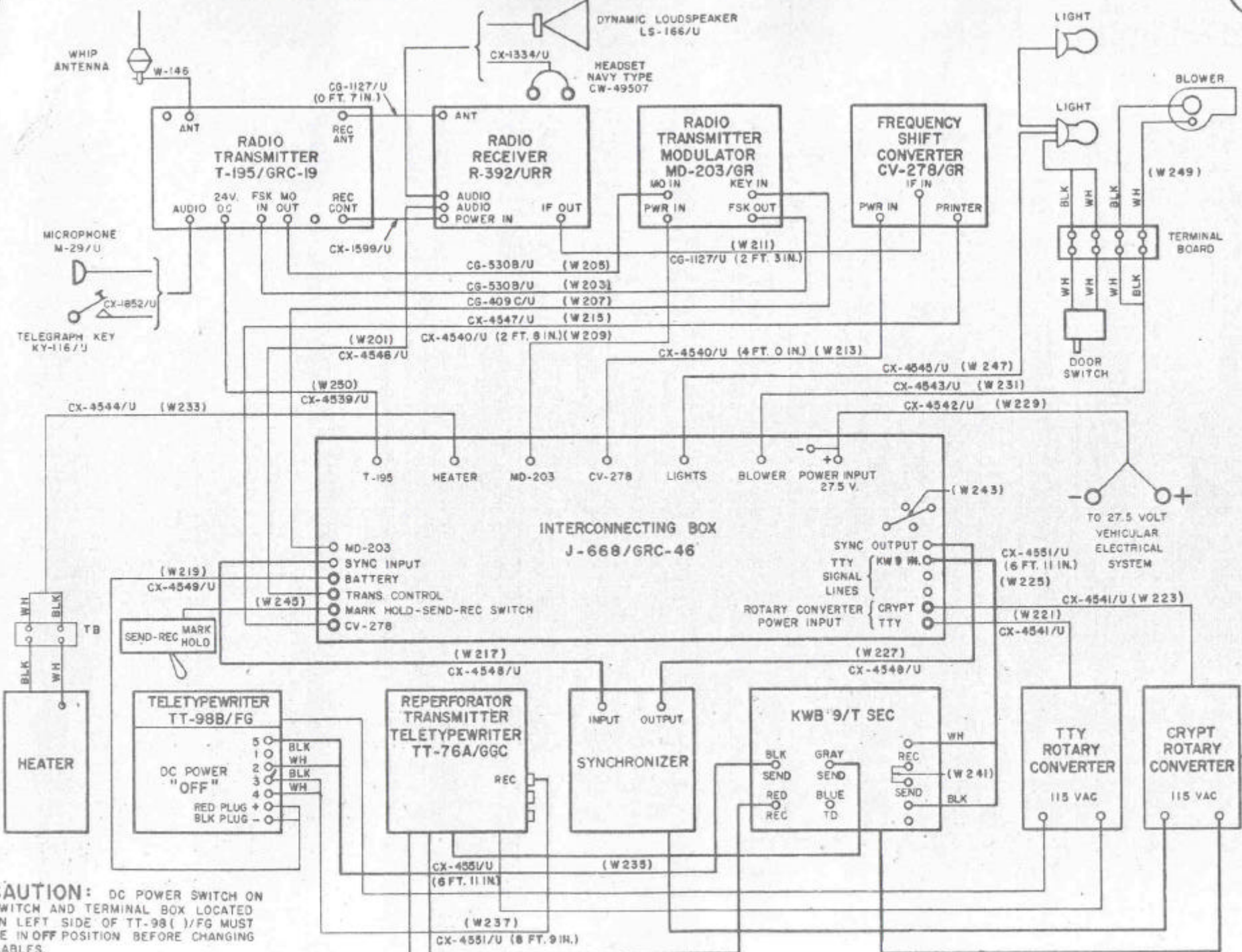
CORDING DIAGRAM AN/GRC-46 ( ) WITH SECURITY EQUIPMENT
