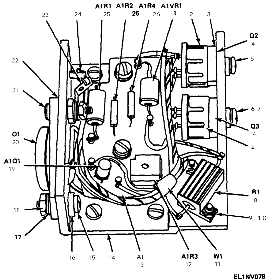
Figure 55. Chassis, Amplifier (2A1A1 ), Voltage Regulator Subassembly (2A1A1A2A2).
