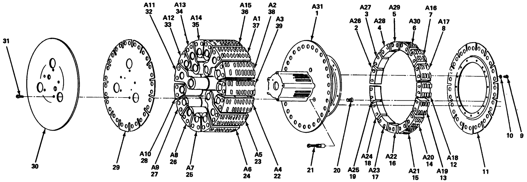
Figure 68. Turret Assembly (2A2) Drum Turret (2A2A1).
